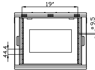
Front View Without the Door
